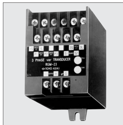
var-TRANSDUCER
